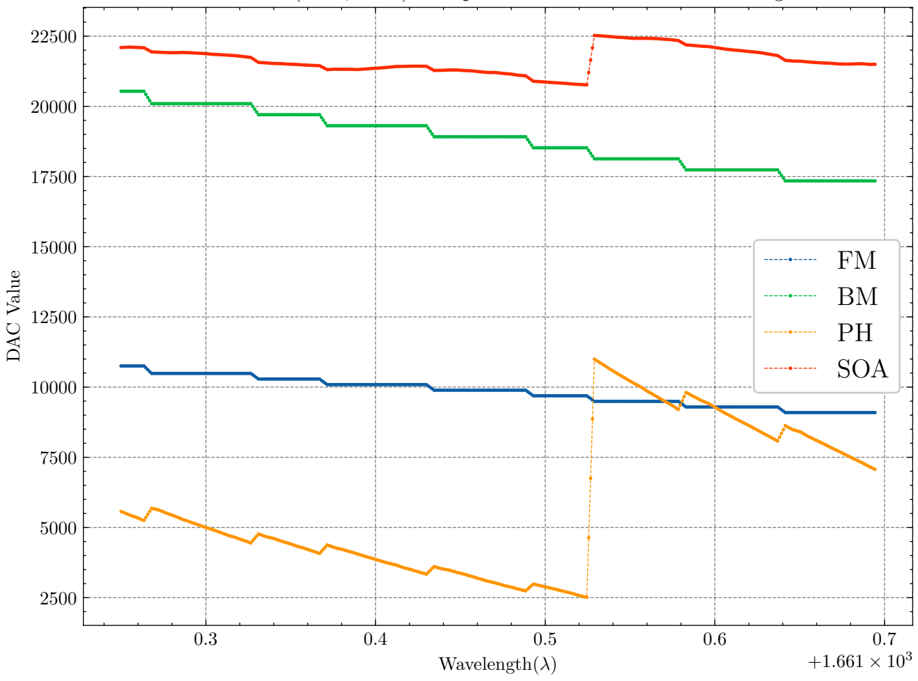
DAC Parameters (7500, 7600) Interpolated with 3 Intermediate Integer Values
